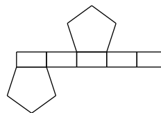
pentagonal prism
