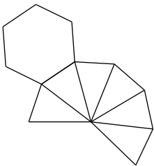
hexagonal pyramid
